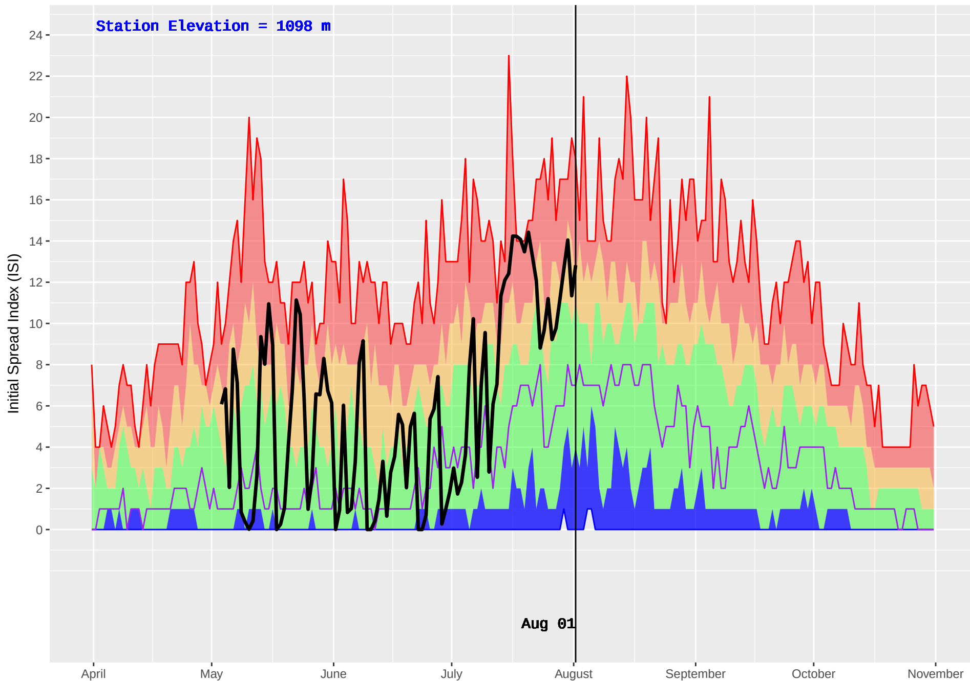
GOATFELL (401) : Historical (1986–2016) and Current (2018) Daily Initial Spread Index (ISI)
