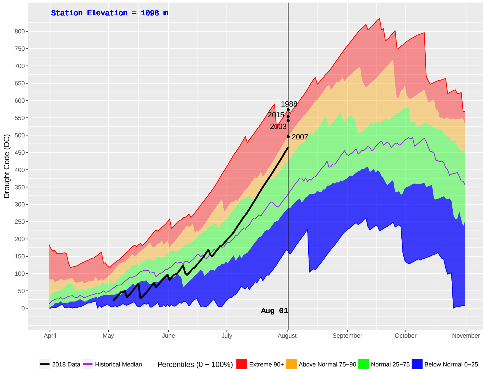
GOATFELL (401) : Historical (1986–2016) and Current (2018) Daily Drought Code (DC)
