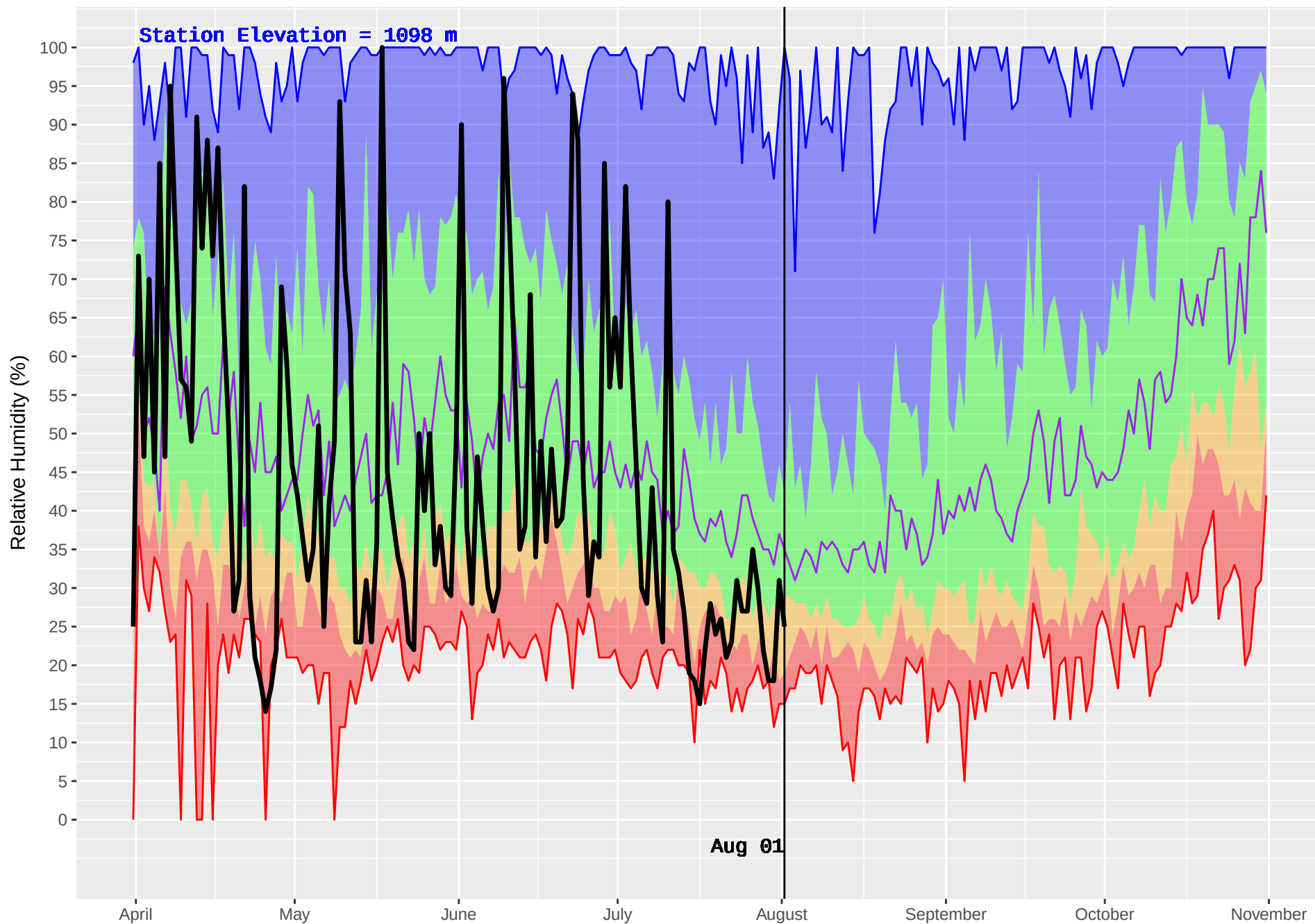
GOATFELL (401) : Historical (1986–2016) and Current (2018) Daily Relative Humidity
