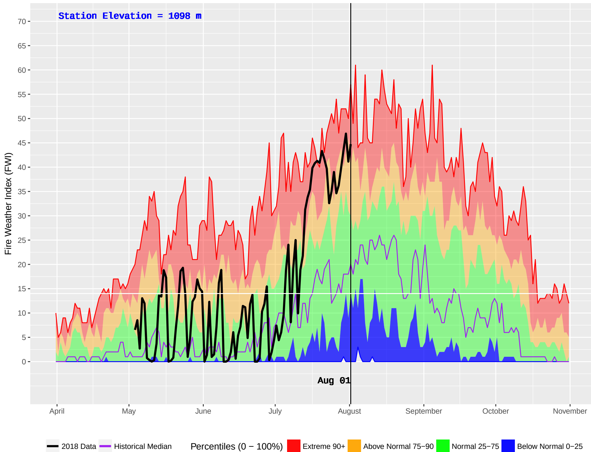
GOATFELL (401) : Historical (1986–2016) and Current (2018) Daily Fire Weather Index (FWI)
