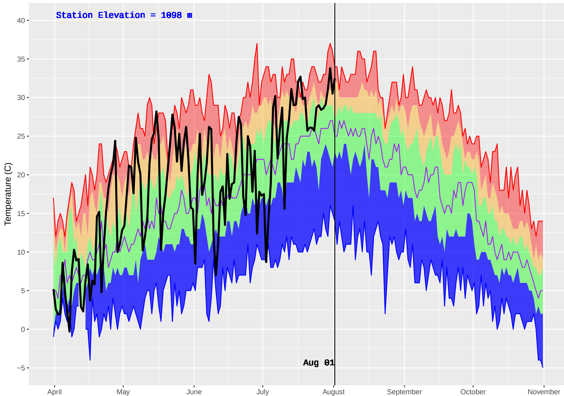
GOATFELL (401) : Historical (1986–2016) and Current (2018) Daily Temperature
